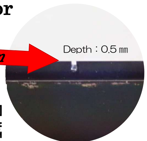
Joints made by Gun-Type Connecting Tool
